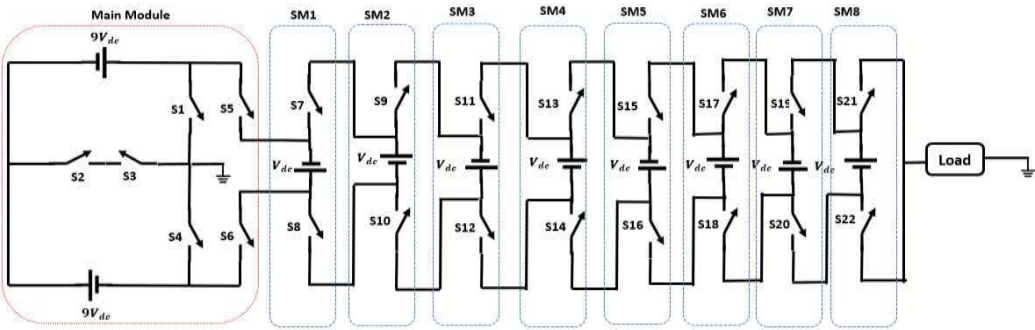
Fig.9 53 level inverter
