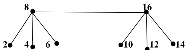
Figure 8: Vertex even mean labeling of P_2 + 2S_3
