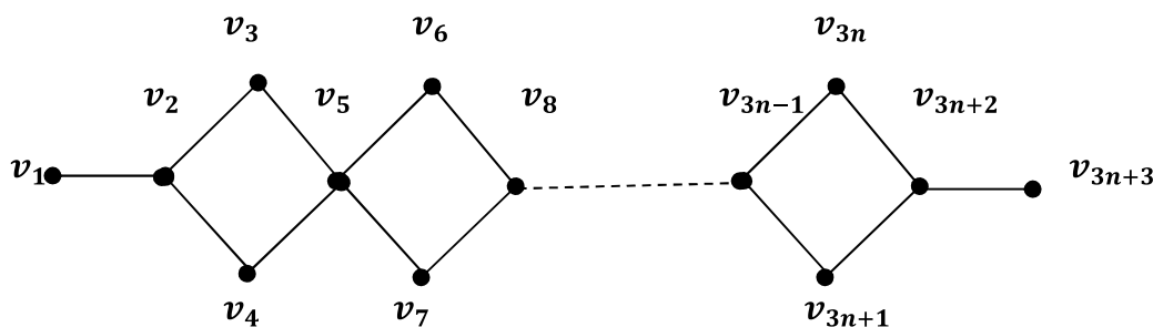
Figure 3: Vertex odd mean labeling of nC_4+2P_2
