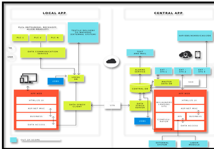
Figure 3: Plant Operational Platform architecture
